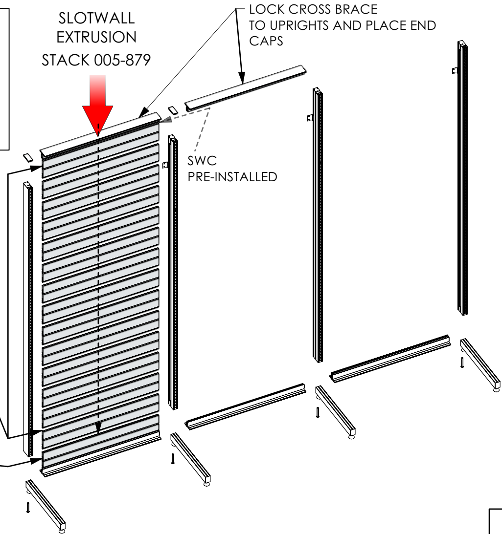
SLOT WALL BOTTOM CHANNEL
